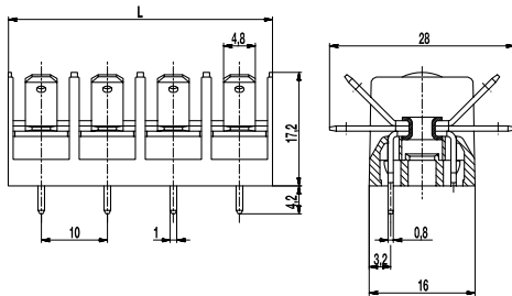
L = Number of poles x pitch Terminal design with tab connector package 8.022
